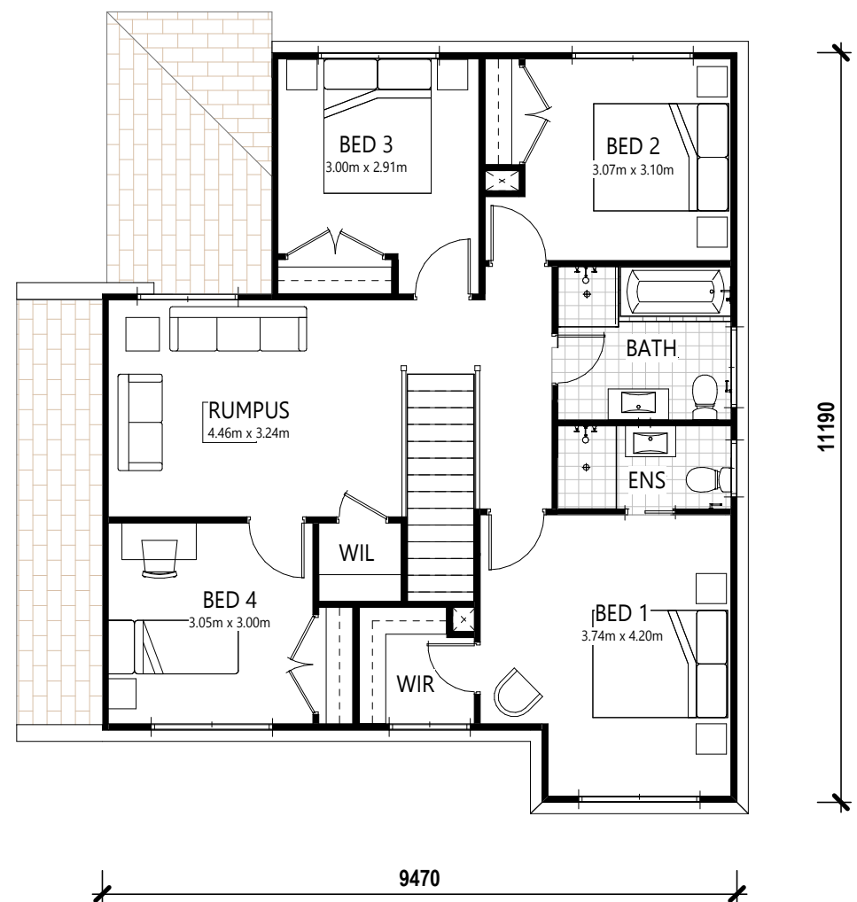
2 UPPER FLOOR PLAN SCALE: 1 : 100
