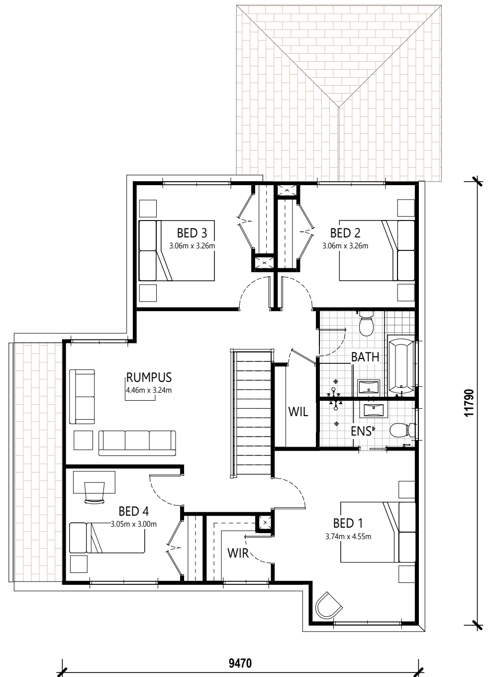
2 UPPER FLOOR PLAN SCALE: 1 : 100
