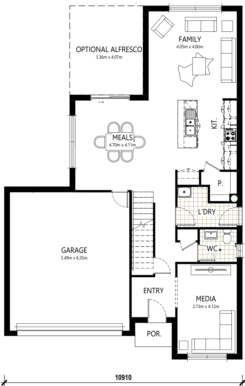
1 LOWER FLOOR PLAN SCALE: 1 : 100
