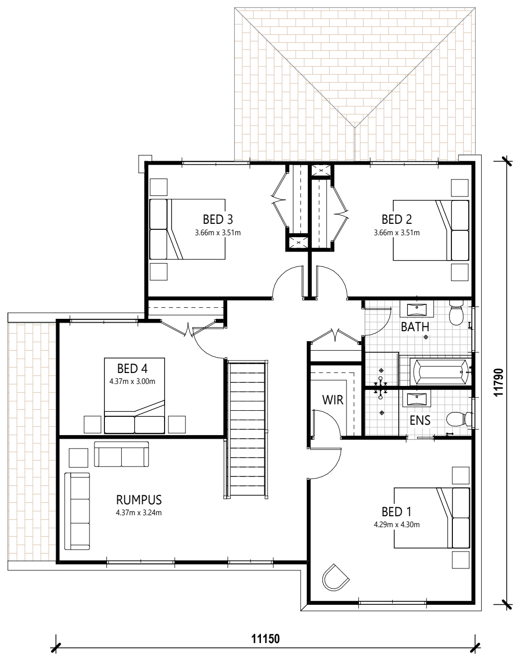
2 UPPER FLOOR PLAN SCALE: 1 : 100
