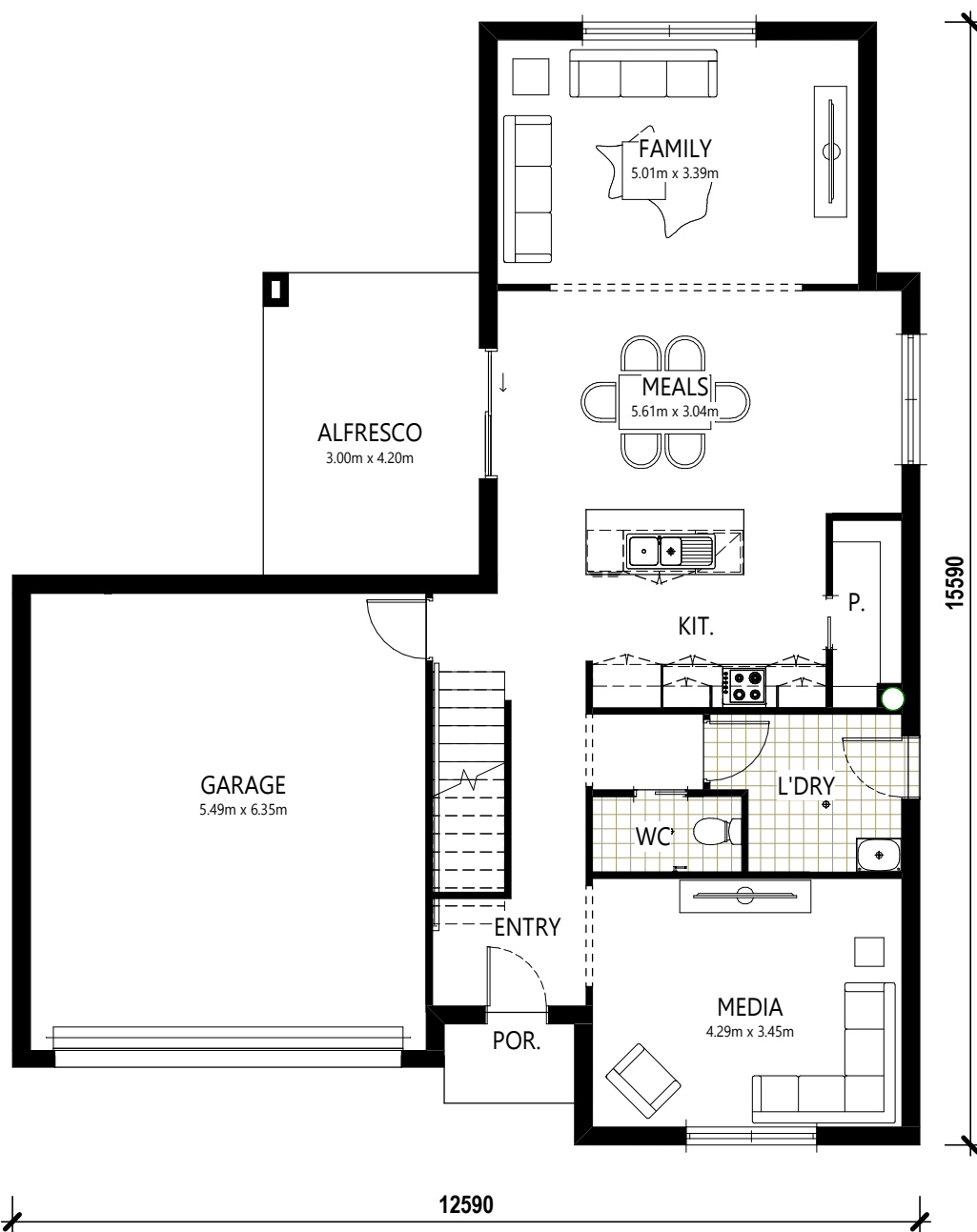
1 LOWER FLOOR PLAN SCALE: 1 : 100
