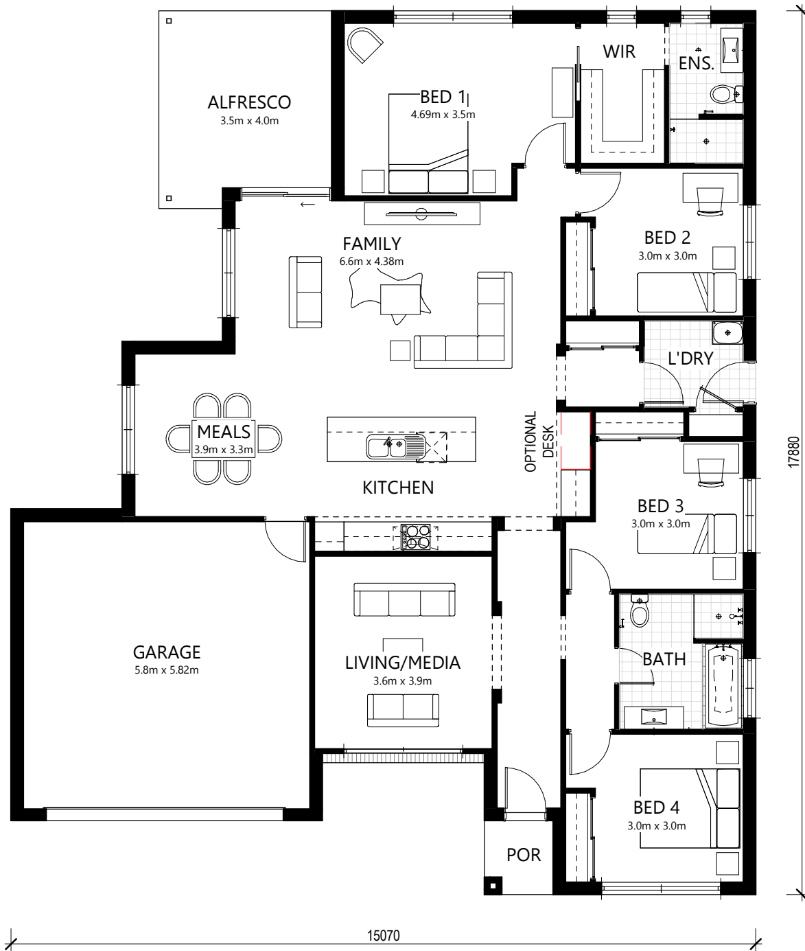
1 FLOOR PLAN SCALE: 1 : 105
