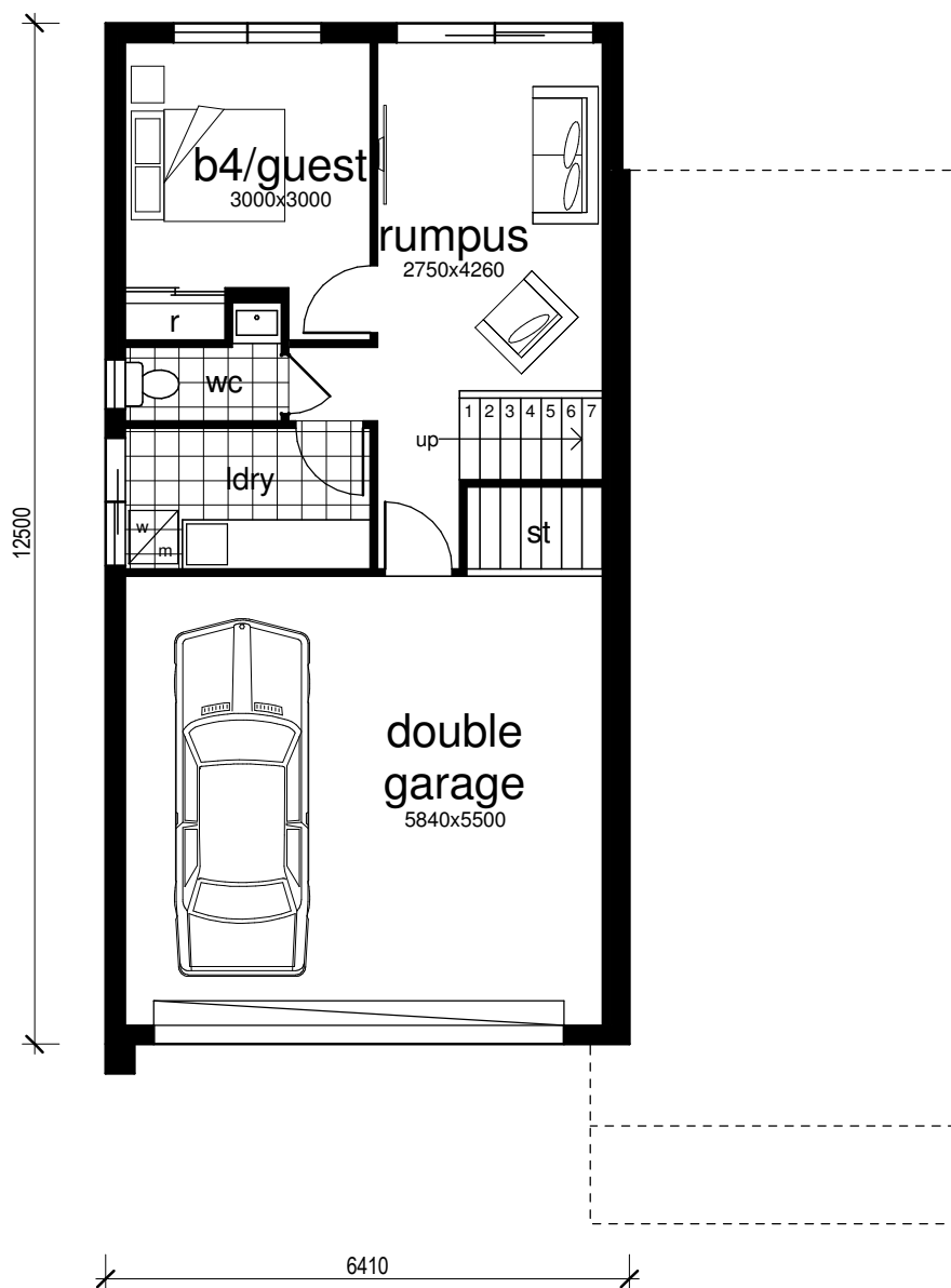
1 GROUND FLOOR SCALE: 1 : 100
