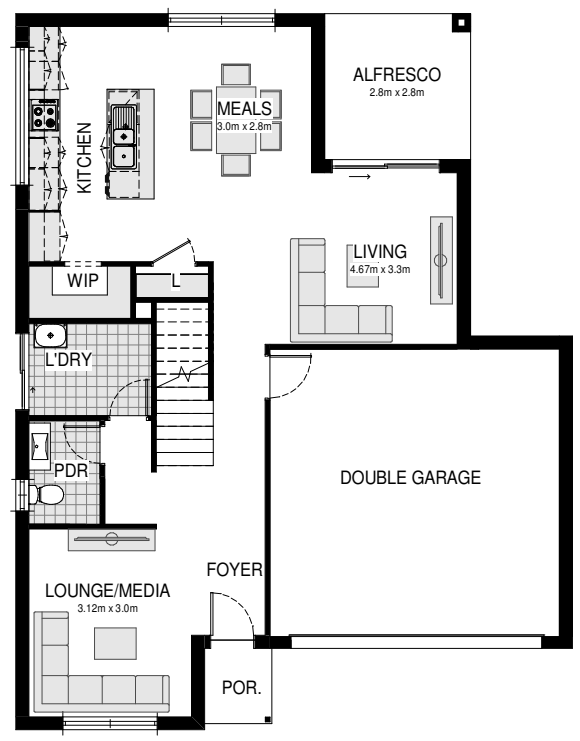
1 LOWER FLOOR PLAN SCALE: 1 : 100
