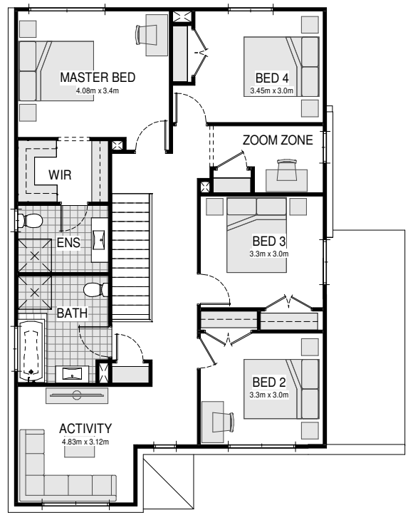
2 UPPER FLOOR PLAN SCALE: 1 : 100
