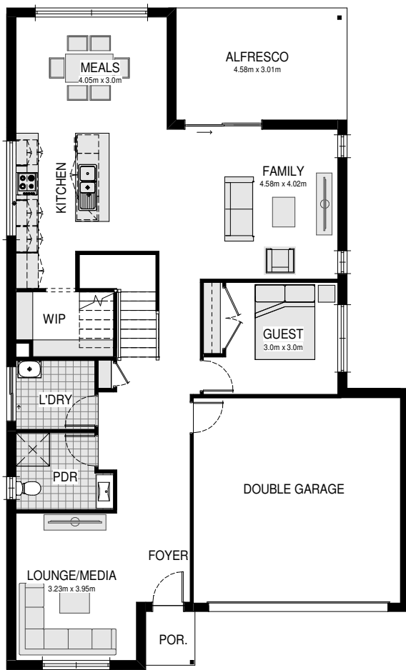
LOWER FLOOR PLAN
