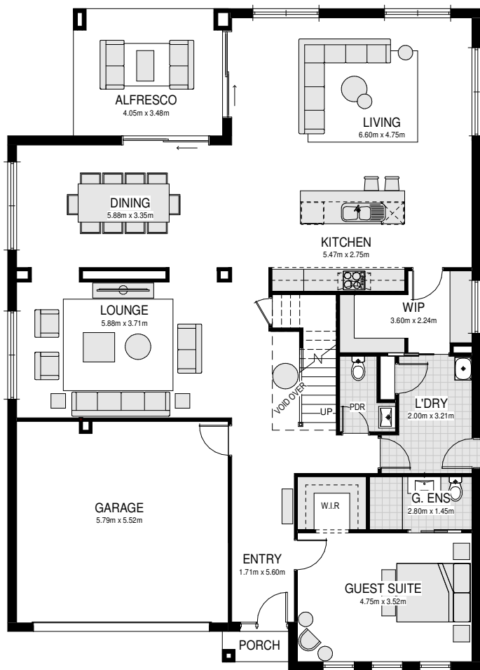
LOWER FLOOR LAYOUT
