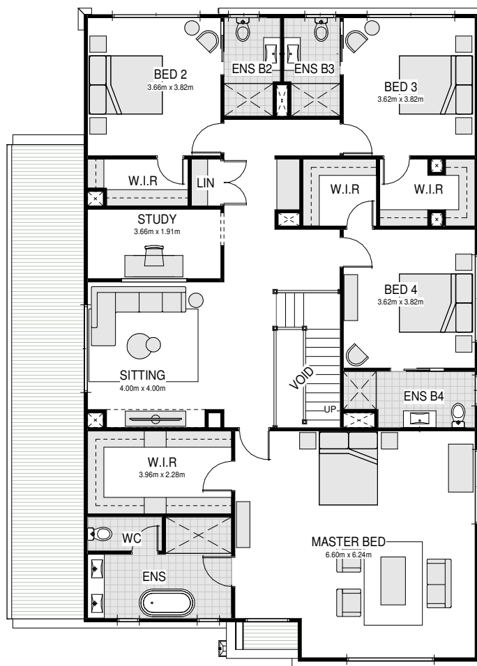
UPPER FLOOR LAYOUT
