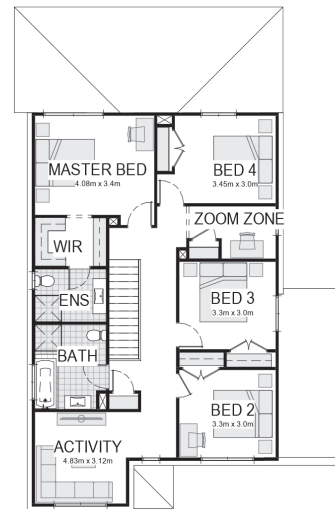
OPTIONAL FIRST FLOOR MASTER TO FRONT
