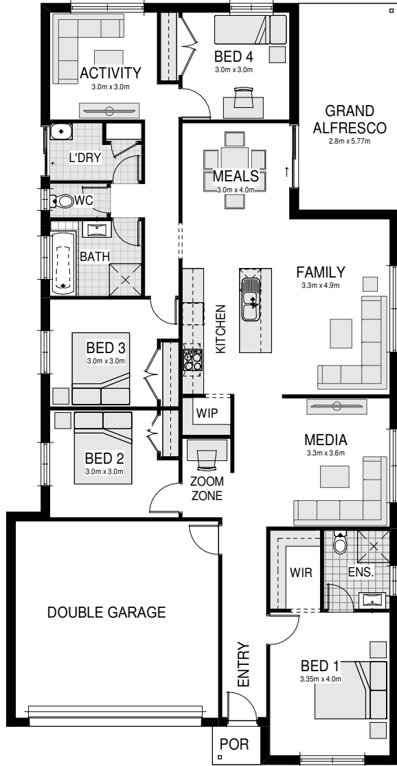
FLOOR LAYOUT
