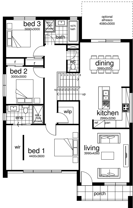
UPPER FLOOR
