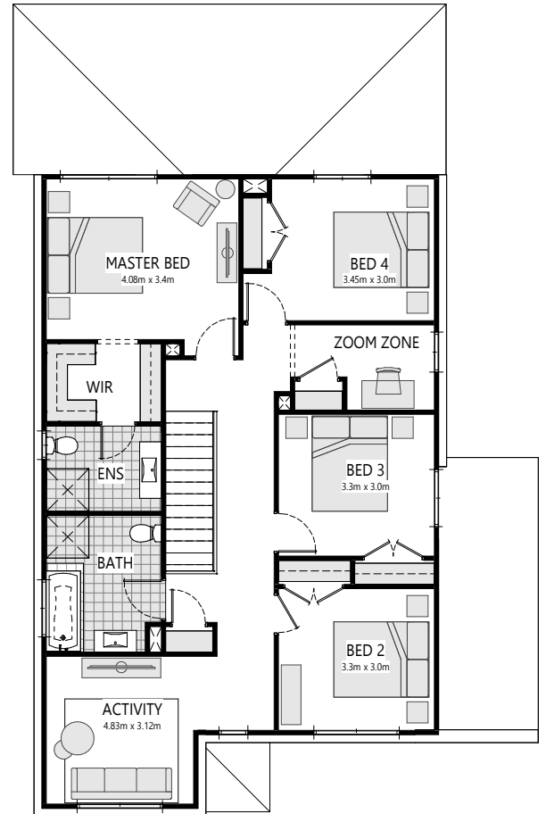
2 UPPER FLOOR PLAN SCALE: 1 : 100
