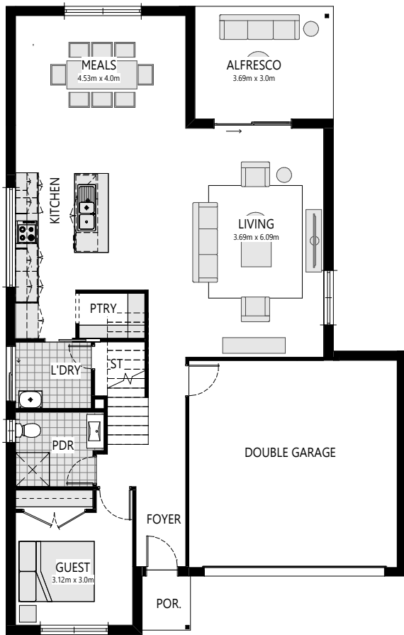
1 LOWER FLOOR PLAN SCALE: 1 : 100
